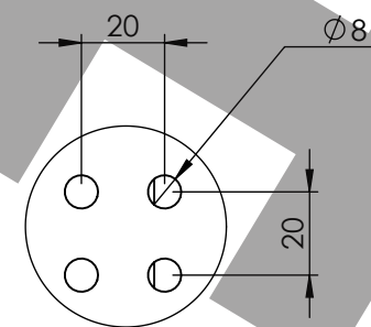
DETAIL K
