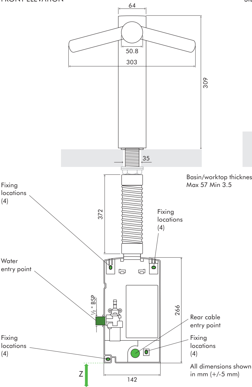
FRONT ELEVATION
