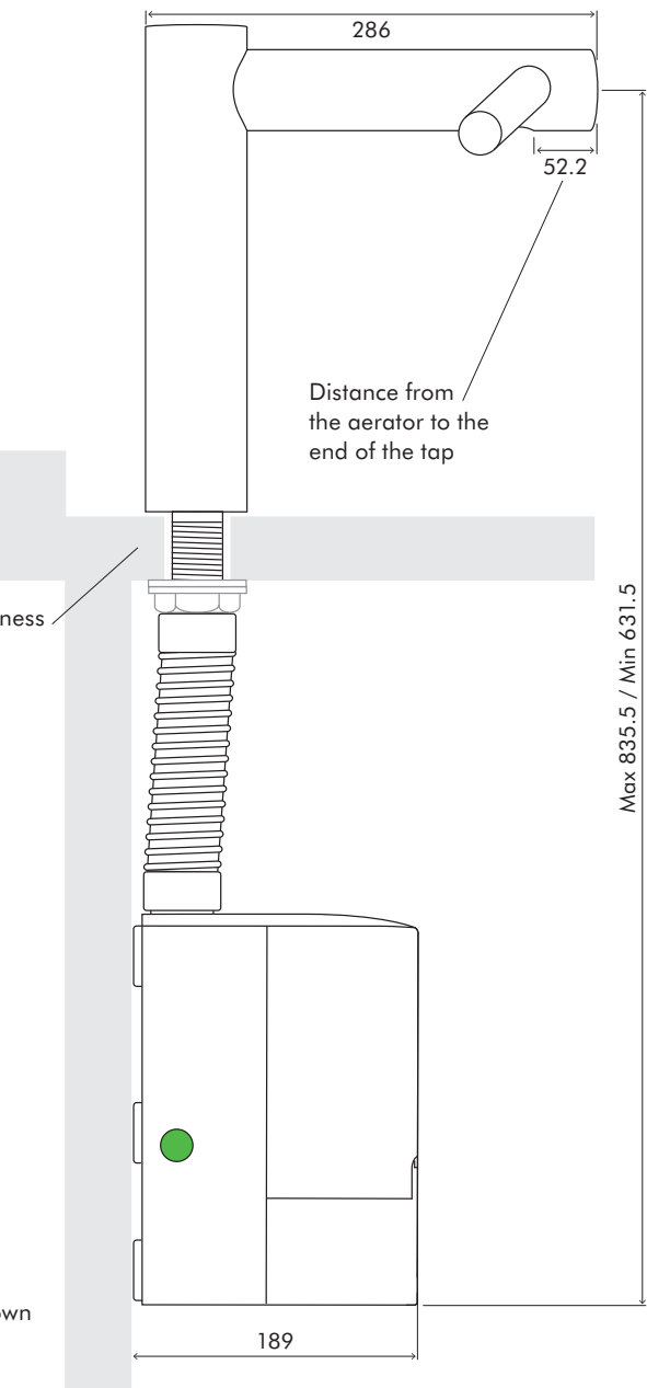
SIDE ELEVATION
