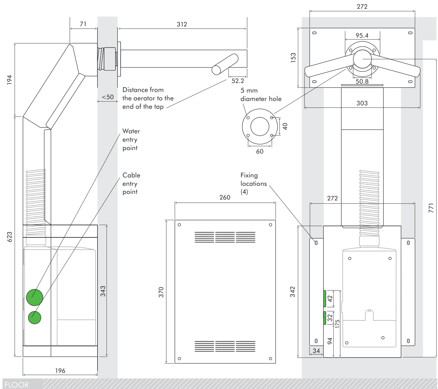
SIDE ELEVATION
